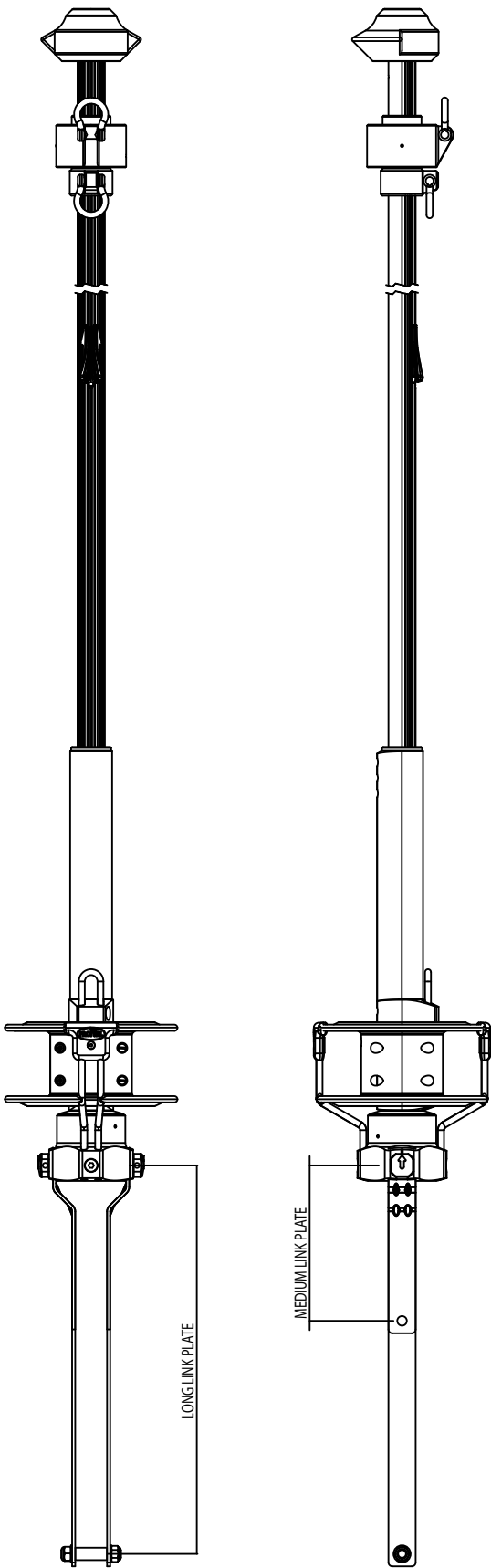
TURNBUCKLE CYLINDER OPTION
